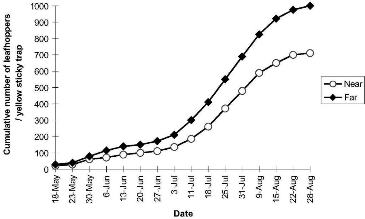
Figure 5. Seasonal patterns of adult leafhoppers in vineyard near and far from the corridor (Hopland, California, 1996).
